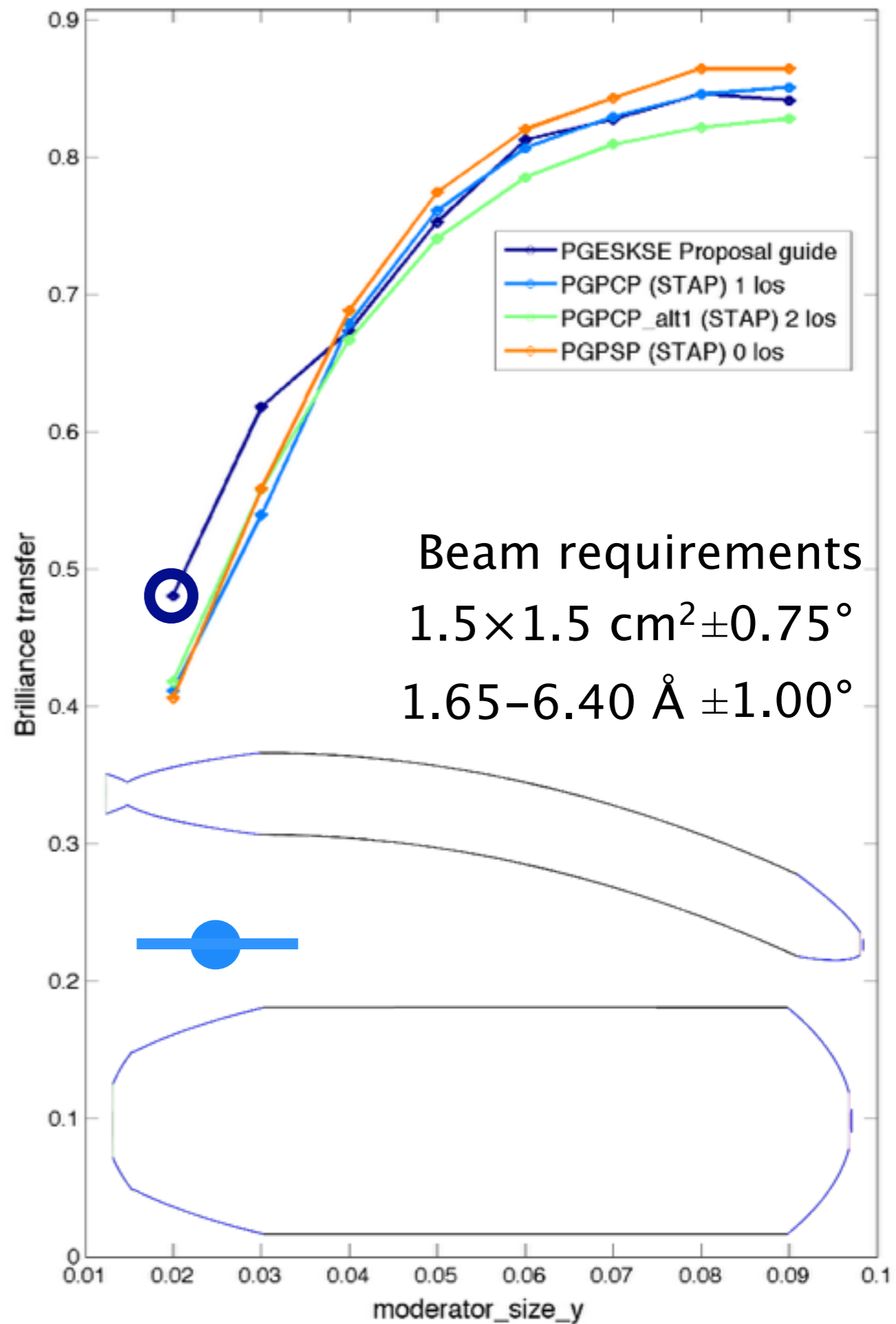
Brilliance Wavelengths = 1.65-6.4 AA
