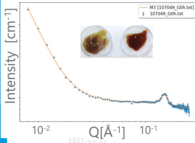
Testing lubricants
