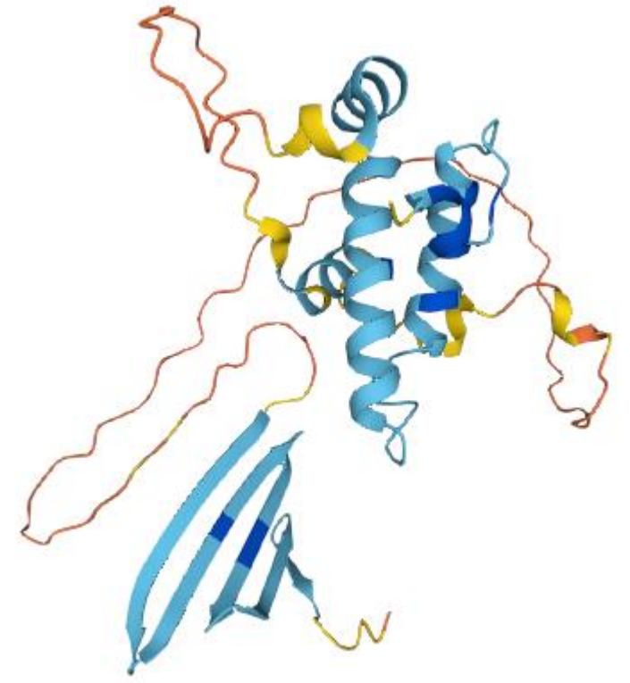
AlphaFold prediction of DNAJB6 structure
