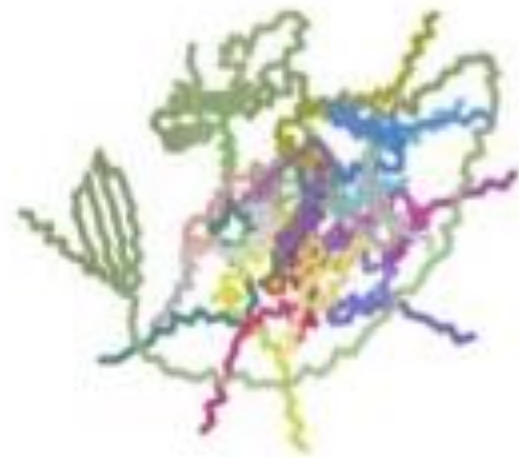
AlphaFold prediction of a DNAJB6 monomer as an \alpha\beta -42 oligomer made up of 16 monomers
