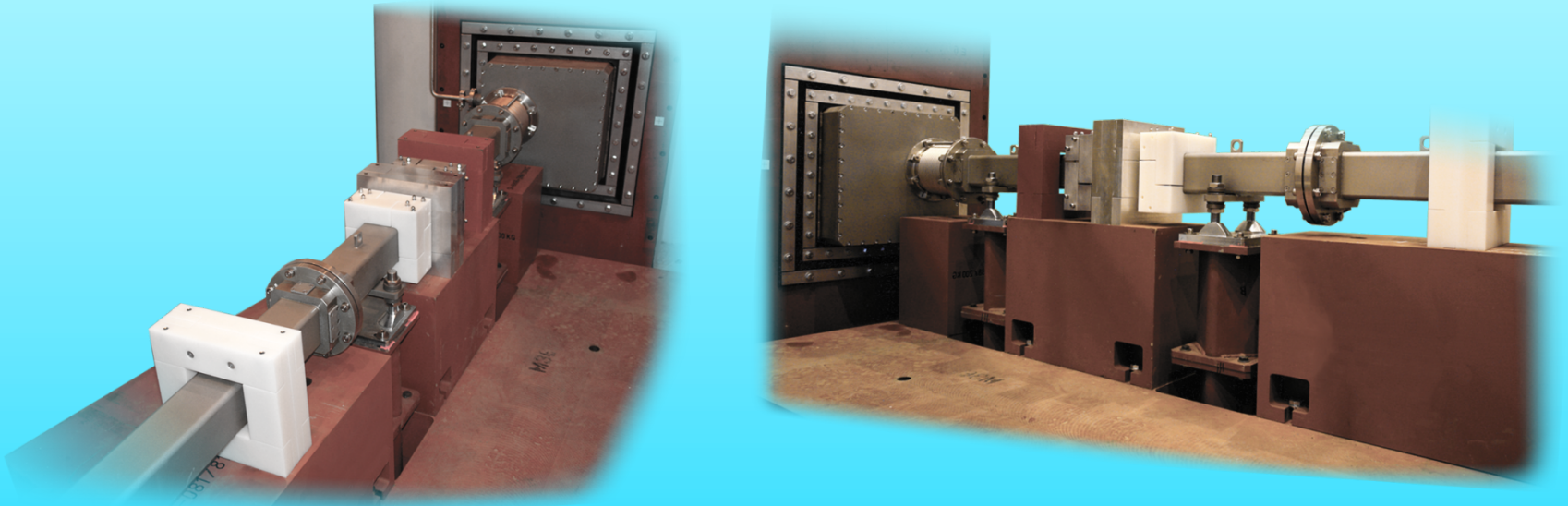
In-pile Insert with guide integrated to Out-of-pile guide system
