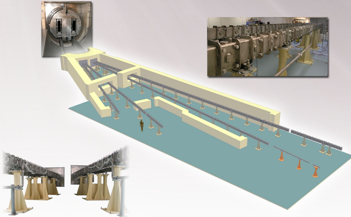
ANSTO 160m long Neutron Guide System
