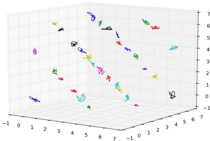
Al 111 plane
