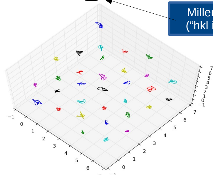
Al 110 plane
