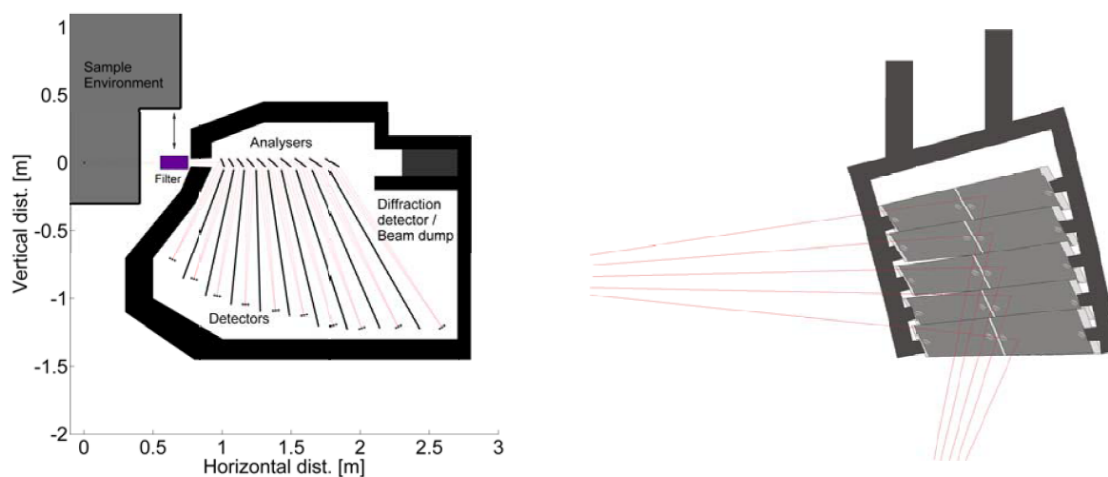
Figure 6 Outline of the spectrometer tank and the analyser setup of BIFROST
