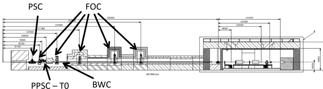
Figure 3, Chopper system layout (to be replaced with BIFROST equivalent)
