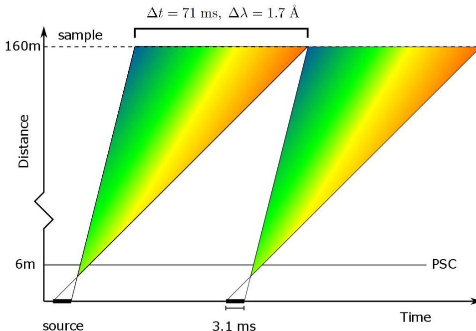
Figure 4. Basic principle of the chopper relevant for the resolution of the BIFROST primary instrument.
