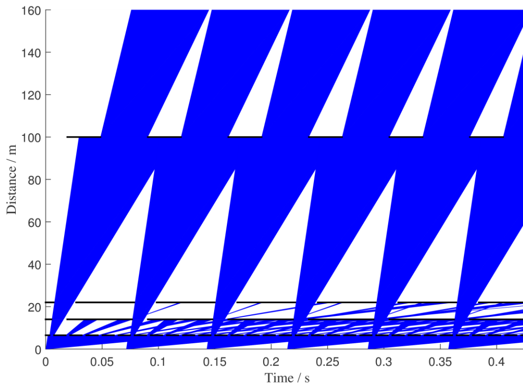
Figure 5 The full chopper system of BIFROST, to scale
