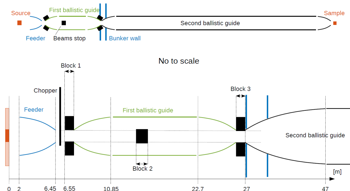
Figure 2, Guide and prompt pulse suppression in BIFROST
