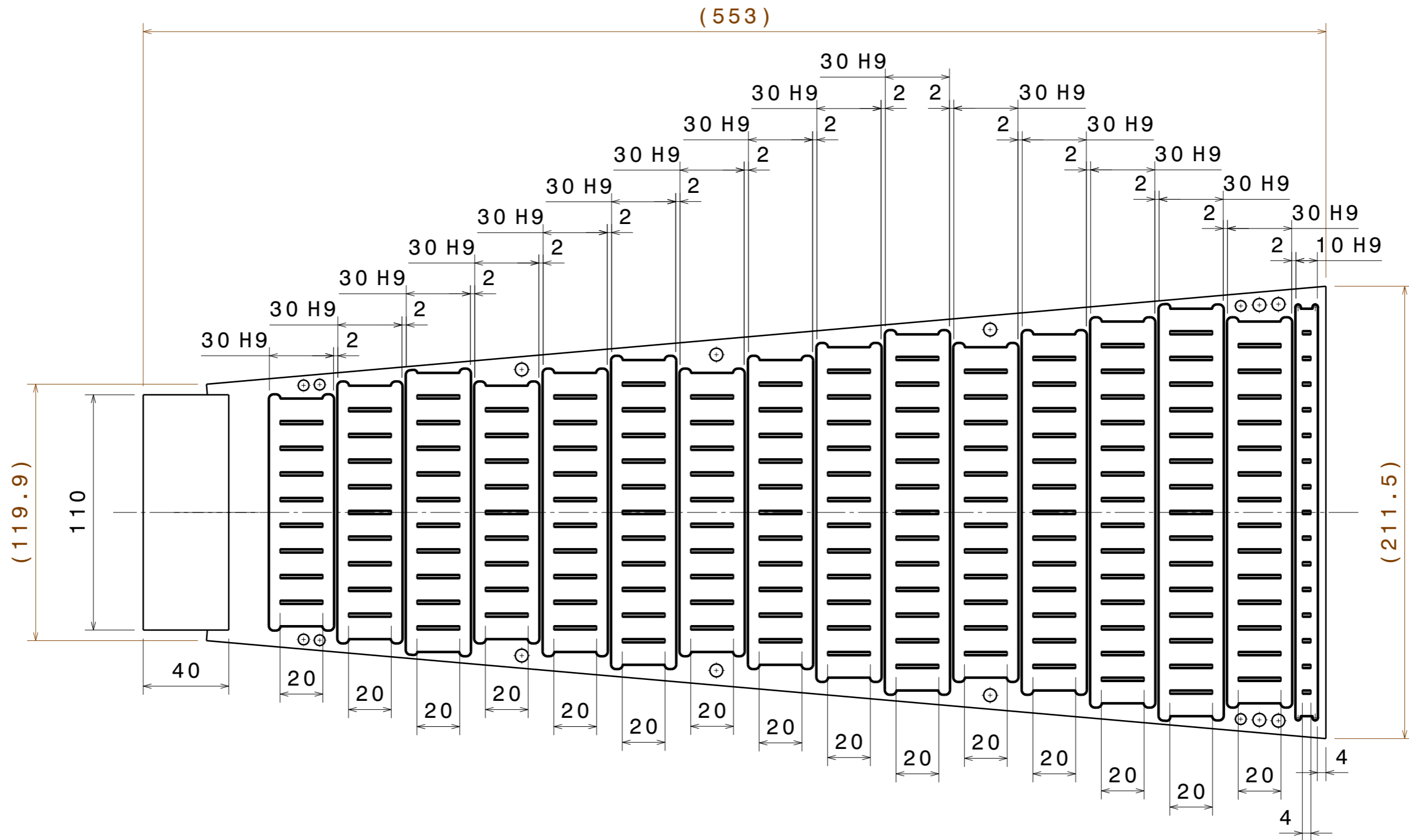
Front view
