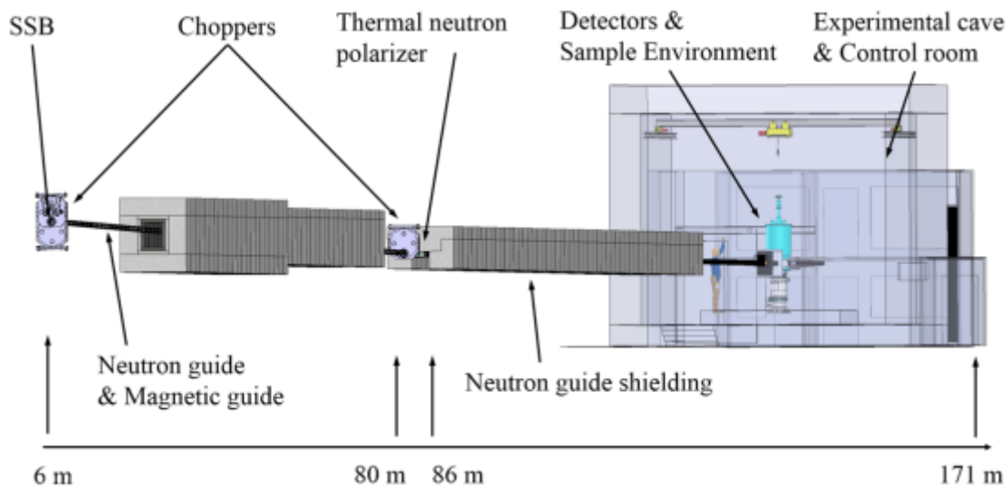
Figure 2. MAGiC conceptual layout
