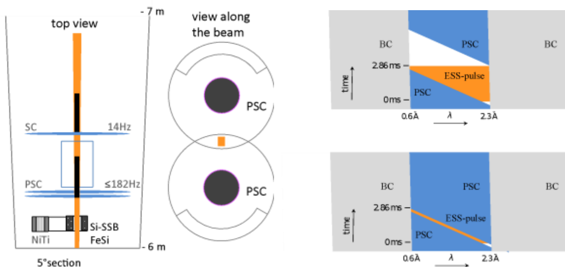
Figure 3 : Pulse Shaping Choppers and Selection Chopper layout
