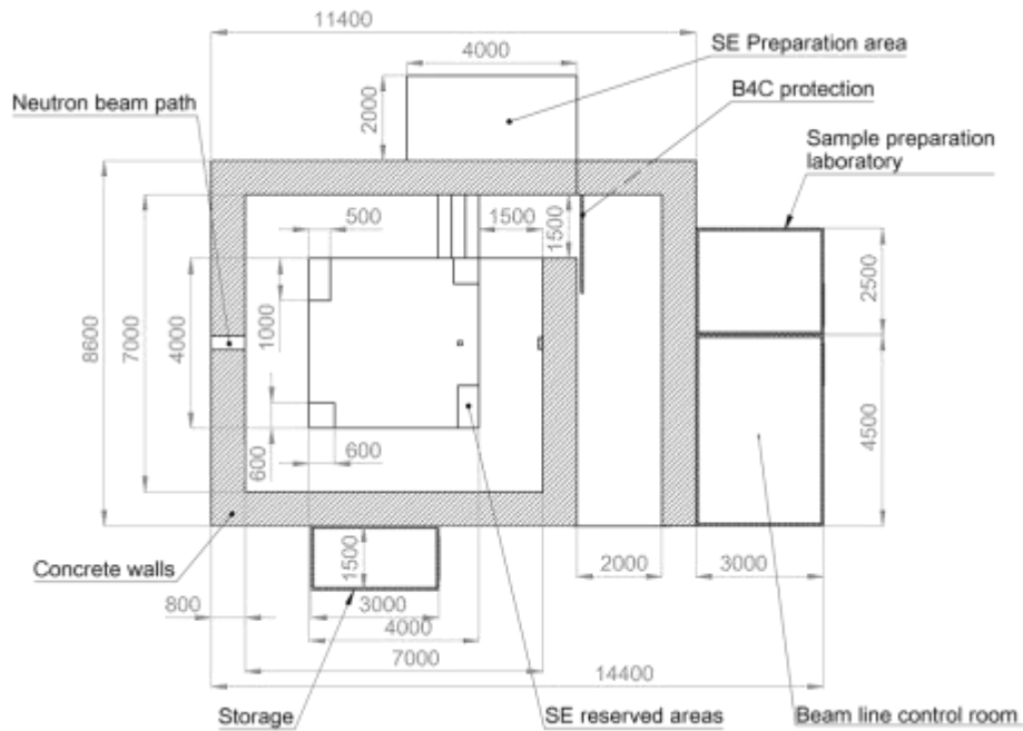
Figure 4: Experimental cave schematic layout
