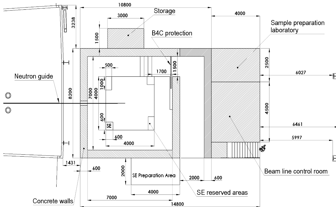
Figure 4: Experimental cave schematic layout
