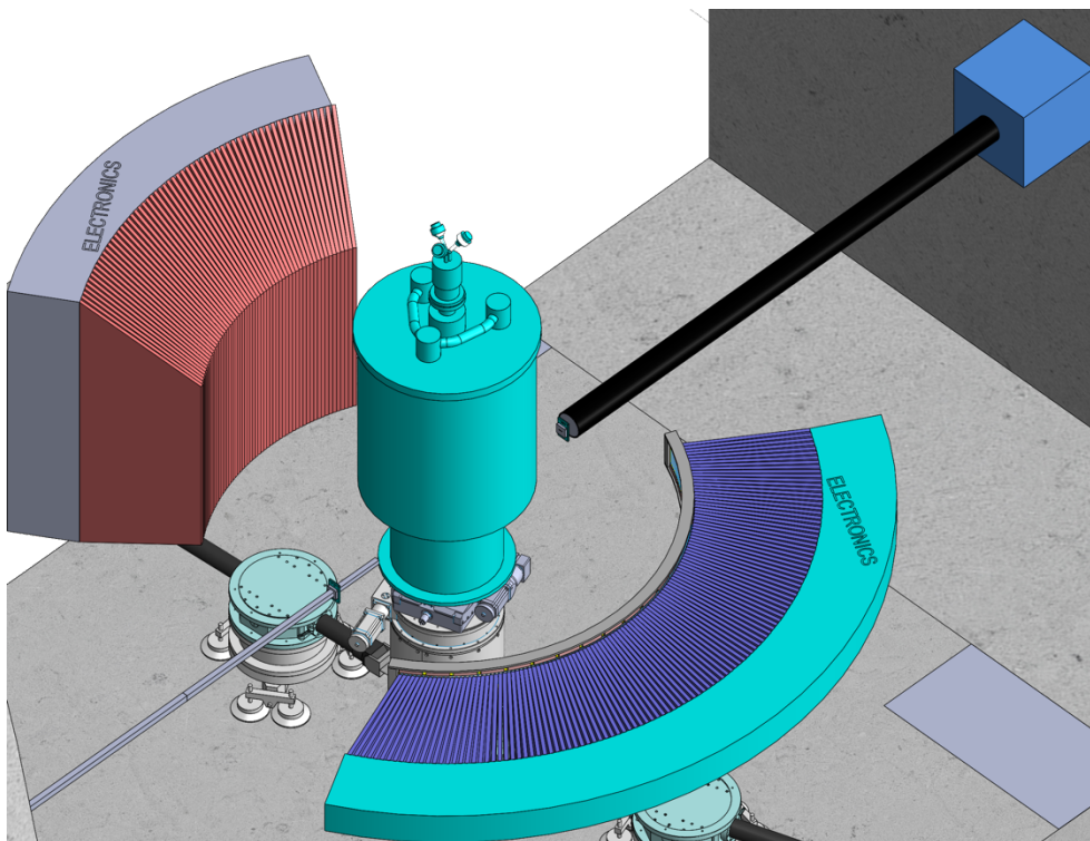
Figure 5: Scheme of the secondary instrument.
