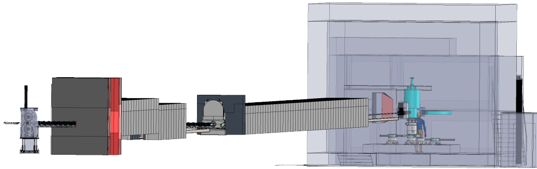
Figure 2. MAGiC conceptual layout
