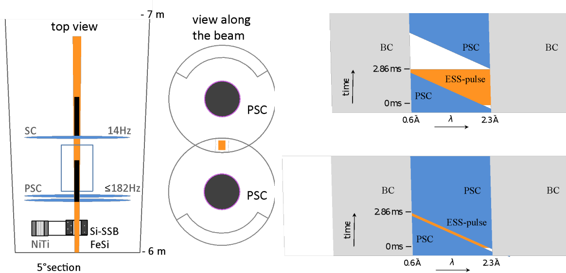
Figure 3 : Pulse Shaping Choppers and Selection Chopper layout
