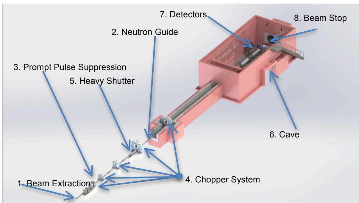
Figure 2. ODIN conceptual layout
