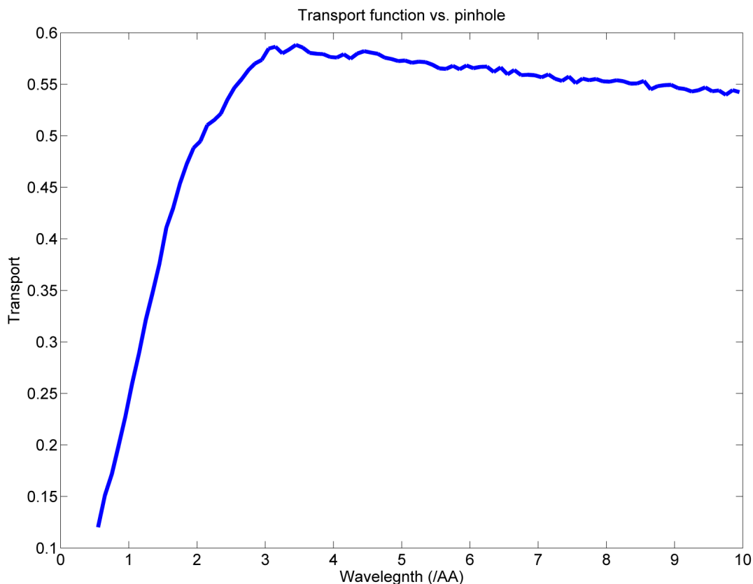
Figure 2: Transport function of the full ODIN neutron optics compared to a pinhole configuration.
