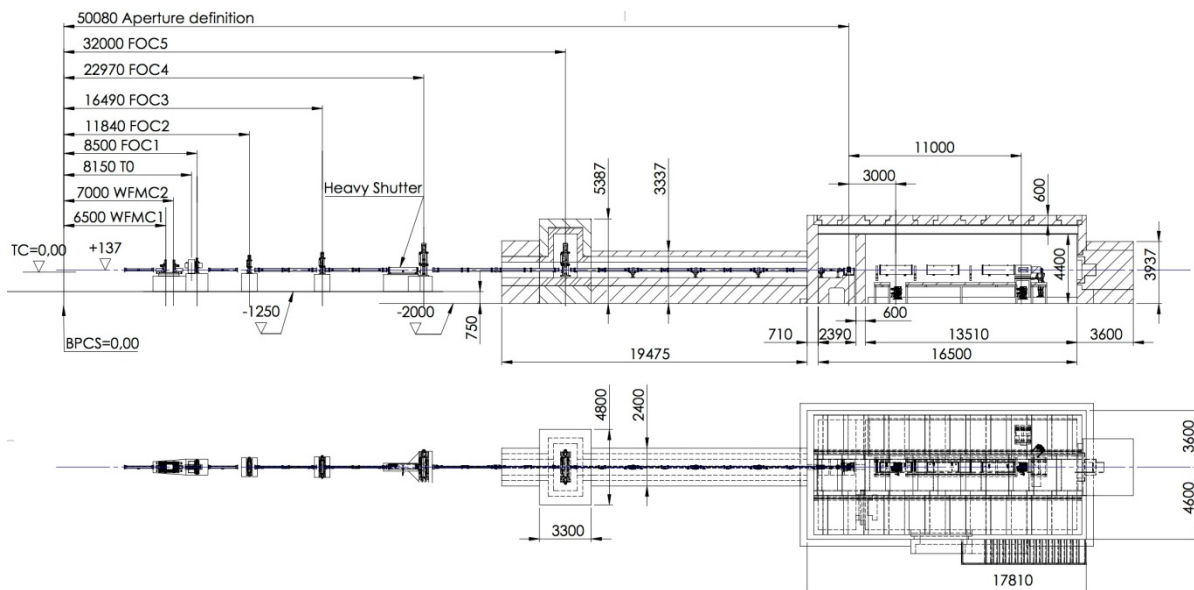
Figure 6. Chopper System Layout
