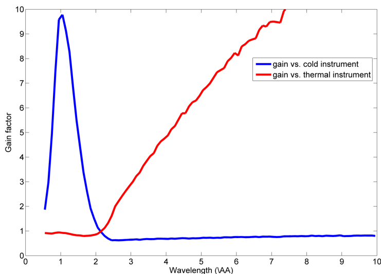
Figure 5. Gain factors by using a bi-spectral extraction on the purely cold and thermal instruments.
