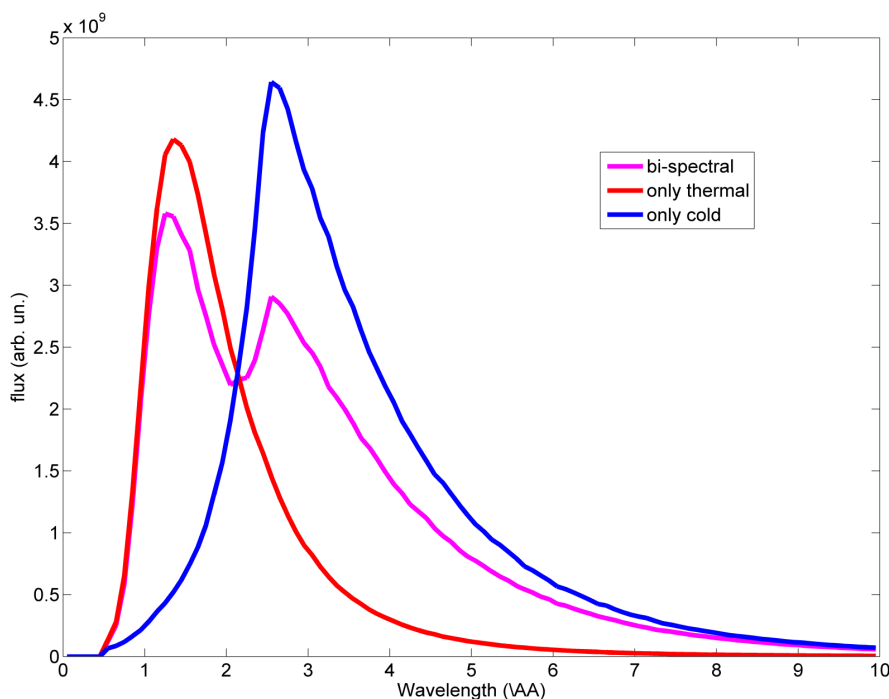
Figure 3: Comparison of the spectra of the current bi-spectral ODIN's optics (pink) to a thermal only (red) and cold only (blue) version of the guide system.
