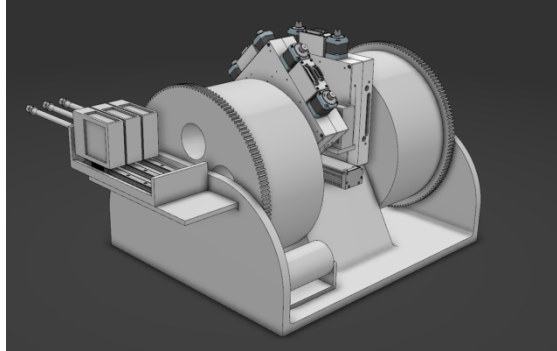
Figure 11: Drawing of the pinhole exchanger.
