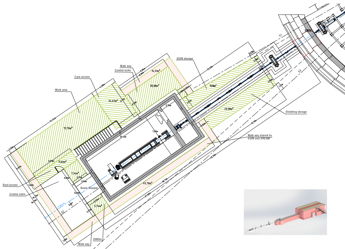
Figure 10: ODIN general layout and floor space plan.
