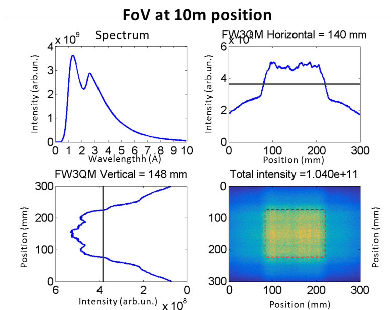
Figure 14. Beam characteristics 10 m from collimator wheel.
