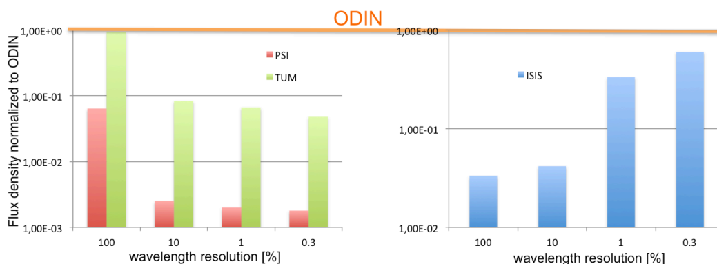
Figure 13. Relative flux comparison, ODIN vs. other state of the art beamlines.
