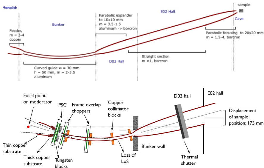
Figure 2, Guide and prompt pulse suppression in Bifrost (sketches). The feeder points to the cold part of the moderator, and the sample position is displaced 175 mm from the beamport axis (horizontal line)
