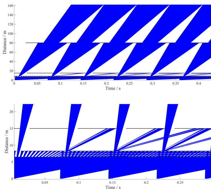
Figure 3 ToF diagram for the chopper system in a worst case setting of maximum speed (210 Hz), maximum opening (2.25 ms). (Top) Full beamline. (Bottom) Bunker and frame overlap. The wavelength interval on the sample position here is 2.95-4.65 Å
