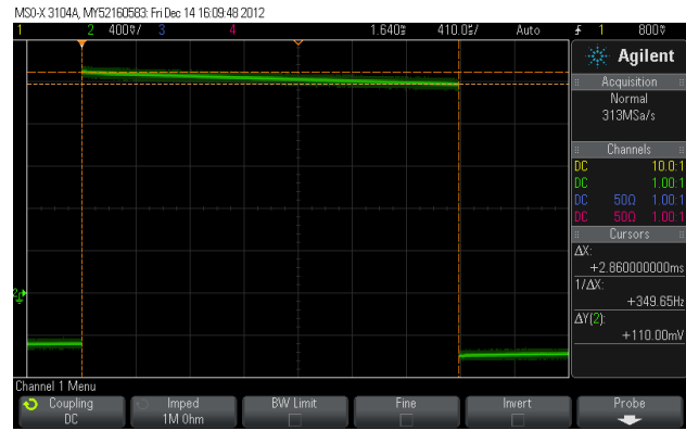
Figure 3: The ACCT droop with a 2.86 ms pulse measured at 4.2%.
