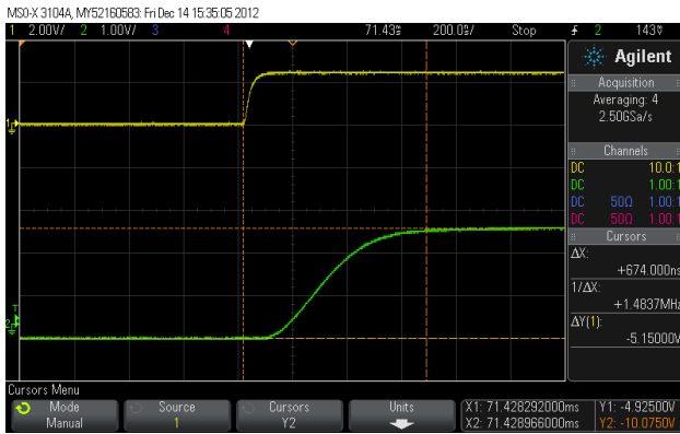
Figure 2: Current pulse (above) and output signal of the ACCT electronics (below) with a settling time of 674 ns.
