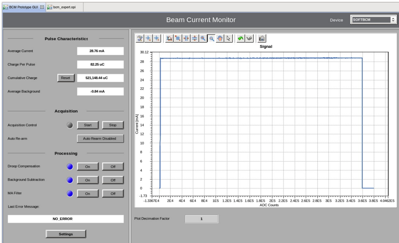
Figure 4: Screenshot of the ACCT GUI showing the current pulse specifications and profile.
