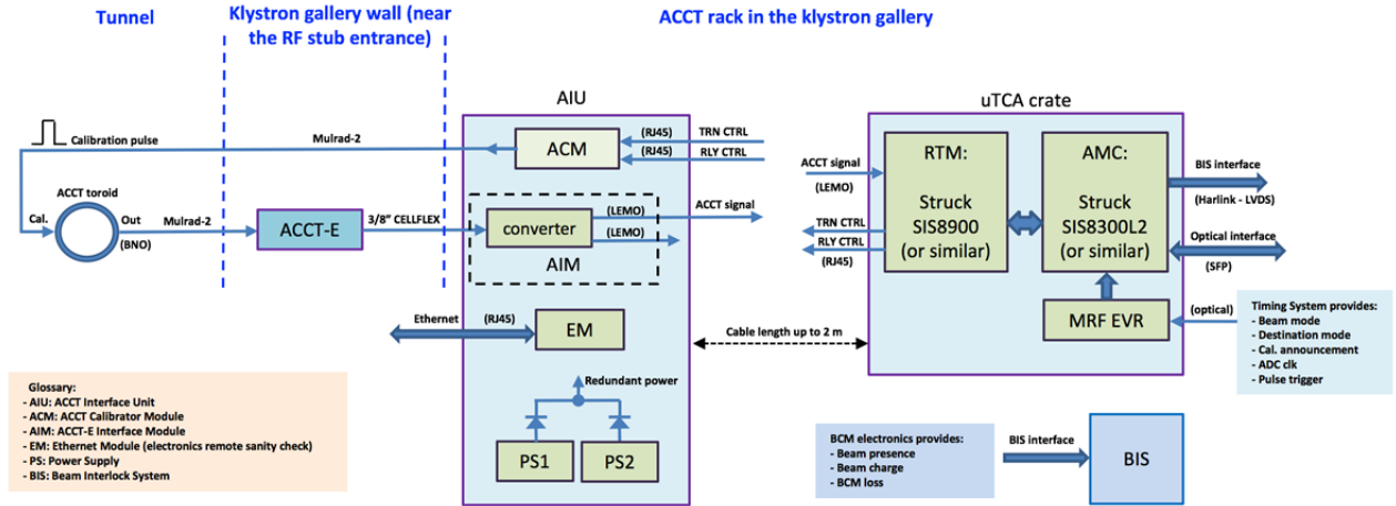
Figure 1: Draft and simplified ACCT layout showing the interconnection of the toroid to the AIU and the crate.
