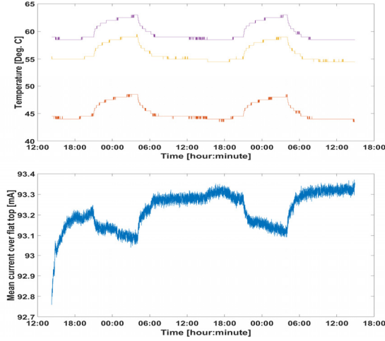
Figure 2: two-day stability test results. Top: measured temperature with 3 sensors in the crate, bottom: history of the measured average current over the pulse flat top.
