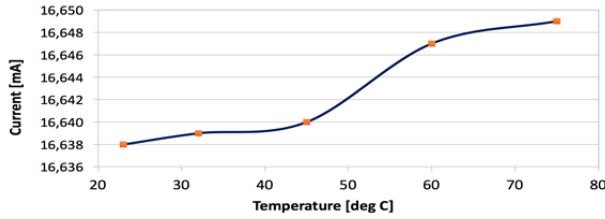
Figure 3: measured ACM drifts with temperature.
