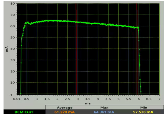
Figure 4: ACCT-measured pulse of the HVPS of the ESS ion source, courtesy of Lorenzo Neri (INFN-Catania) and Oystein Midttun (ESS).
