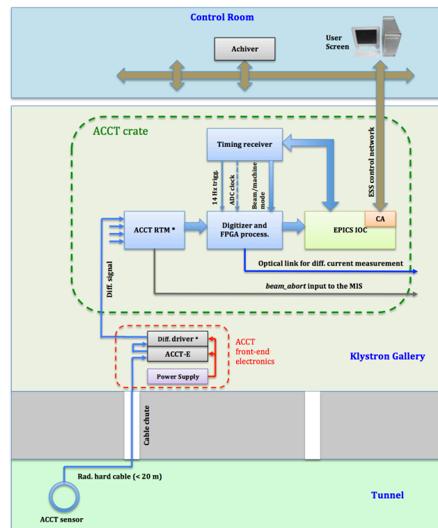
Figure 1: Simplified block diagram of the ACCT system.
