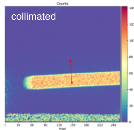
Pixel matrix: 256 x 256 pixels, Pixel pitch: 55 x 55 \mu\text{m}^2
