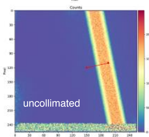
Pixel matrix: 256 x 256 pixels, Pixel pitch: 55 x 55 \mu\text{m}^2
