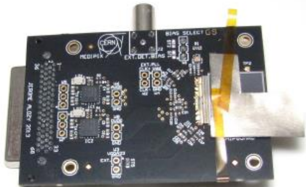
Timepix3 detector with 25um gadolinium foil.
