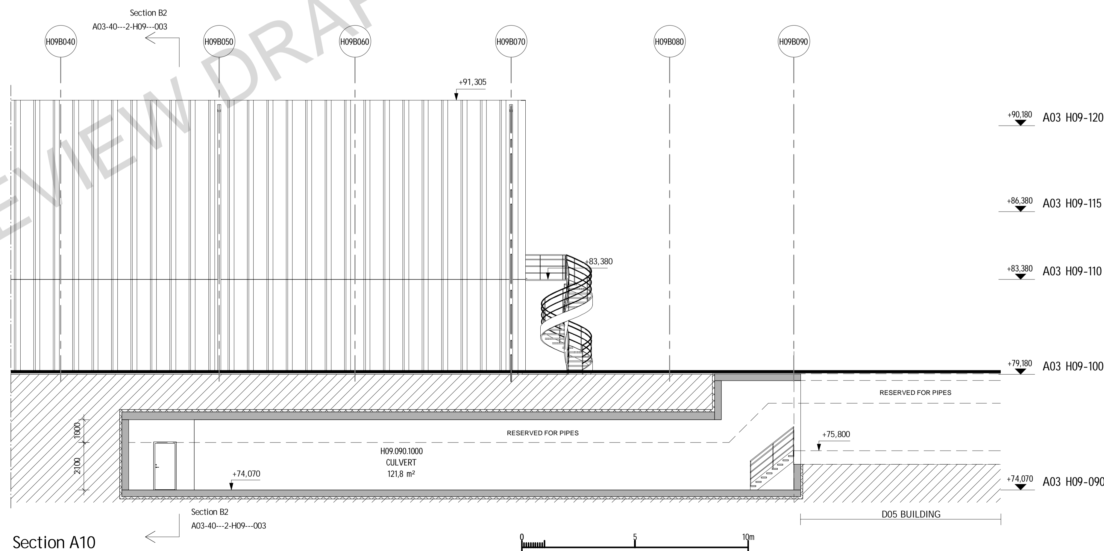
A40 H09-090 CULVERT
