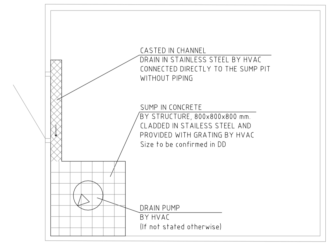
PLAN VIEW ROOM WITHOUT CAST IN PIPES Not in scale
